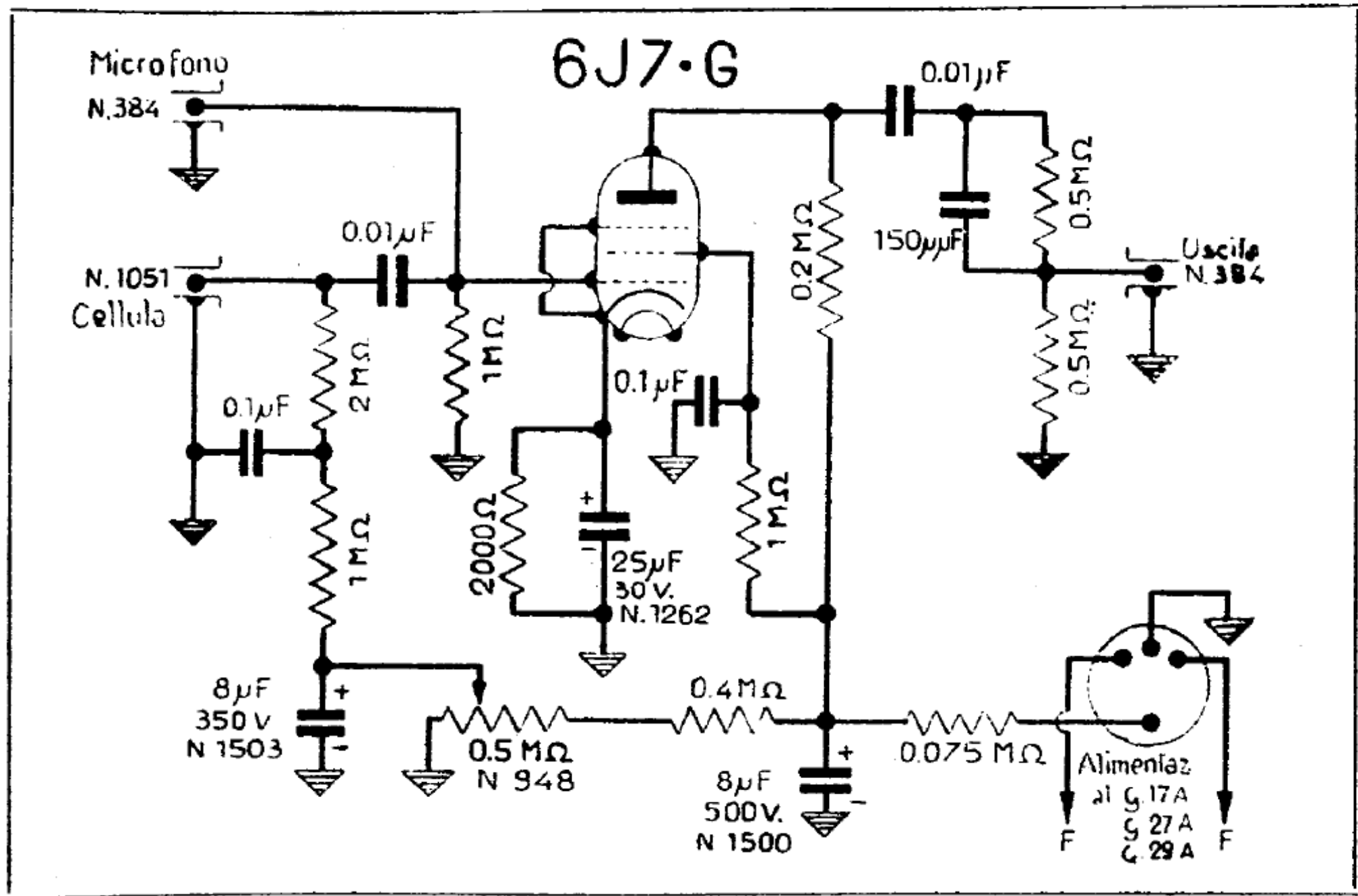
Geloso G1 Preamplifier
